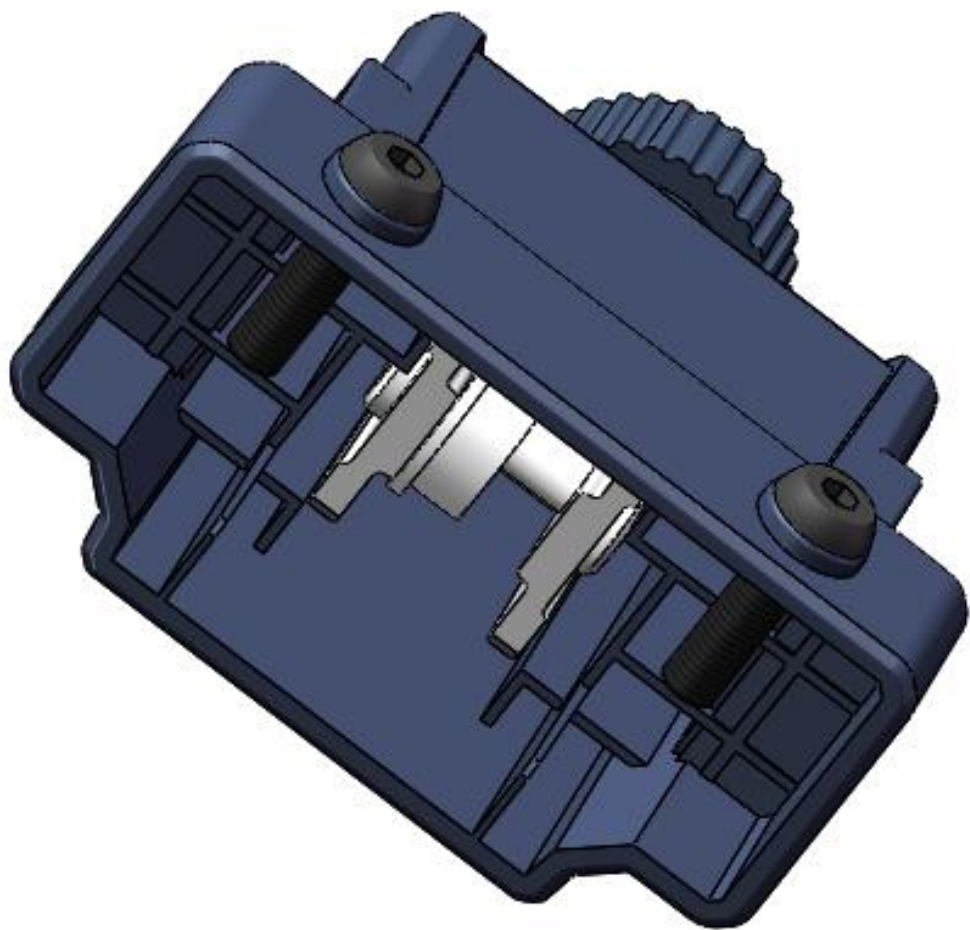
20.204.0124 Y轴皮带调节器组件 Y-Axis Belt Adjustment Assembly
