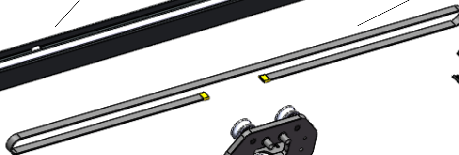
02.203.0066 2020光轴型材-X轴型材 2020 Plain Shaft-X-Axis Profile
