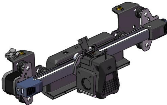
20.203.0046 X轴套件 X-Axis Kit
